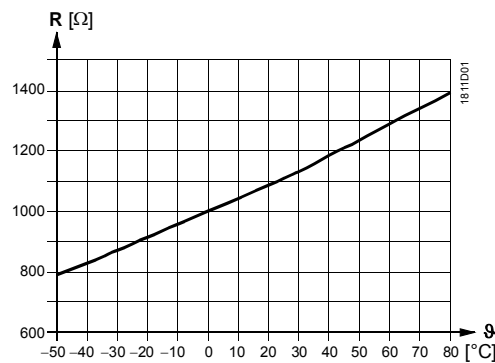
Characteristic LG-Ni 1000
